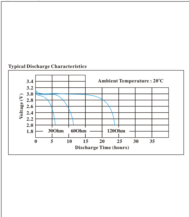
Typical Discharge Characteristics
